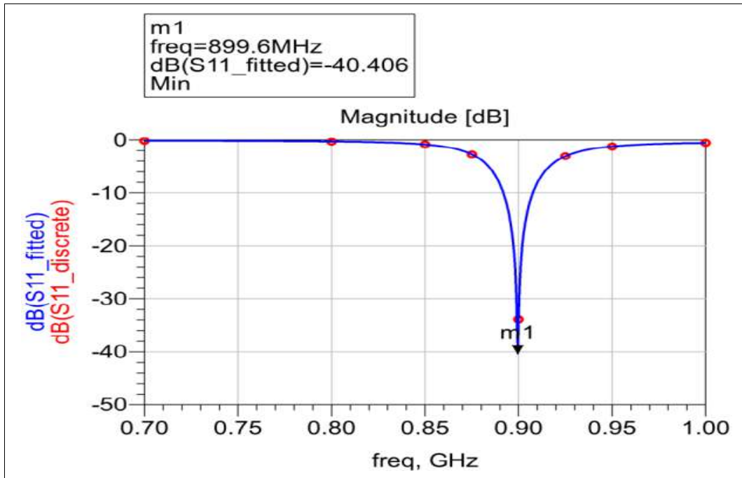
Fig 10: Return loss of 900 MHz patch antenna on rogers-5880 substrate
