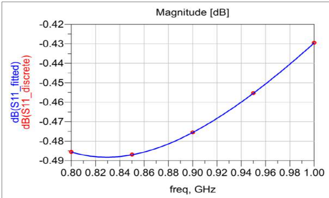
Fig 8: Return loss of 900 MHz patch antenna on fr-4 substrate
