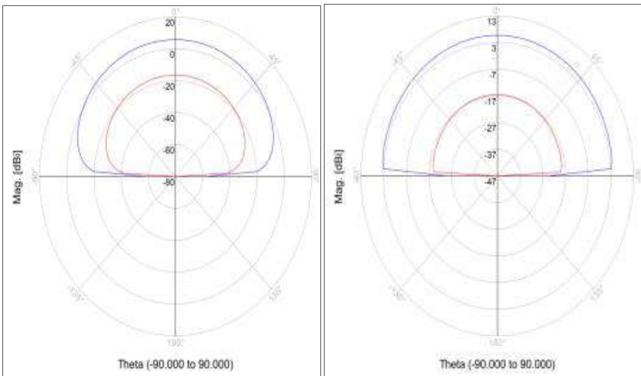
Fig 4: E & H- Field of 900 MHz antenna on fr-4 substrate
