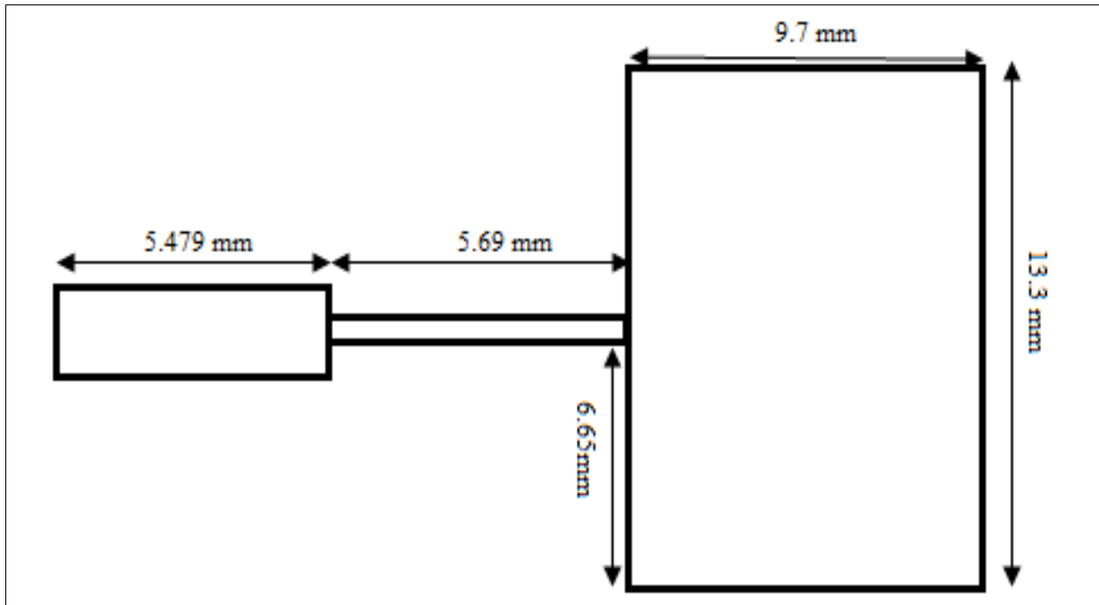
Fig 3: Single patch antenna design layout
