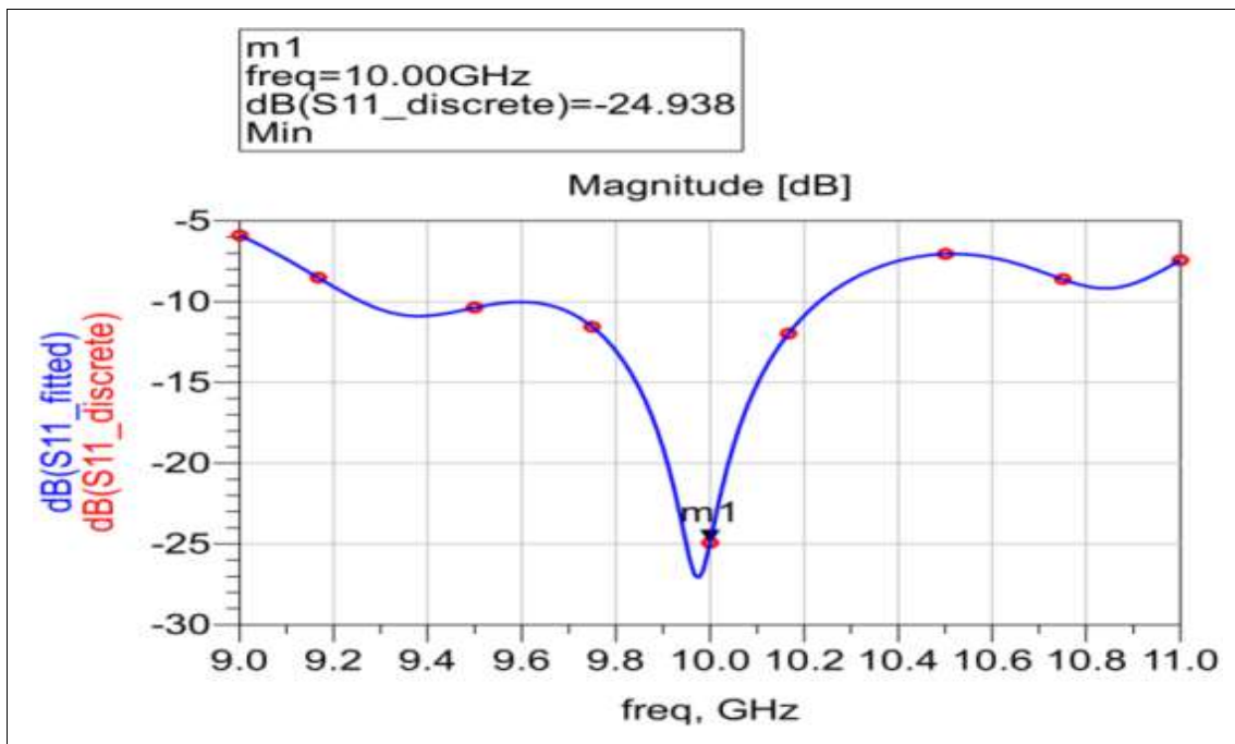
Fig 9: Return loss of 10 GHz patch antenna on fr-4 substrate
