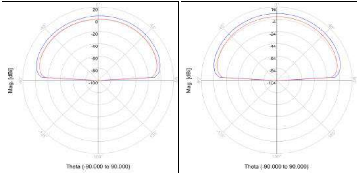
Fig 5: E & H- Field of 10 GHz antenna on fr-4 substrate
