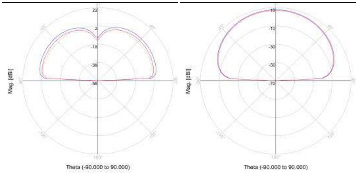
Fig 6: E & H- Field of 900 MHz antenna on rogers-5880 substrate
