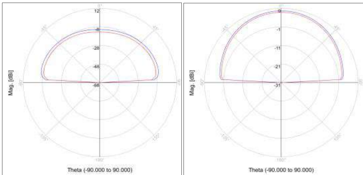
Fig 7: E & H- Field of 10GHz antenna on rogers-5880 substrate
