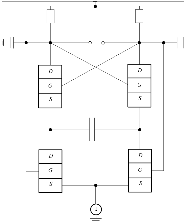
Fig 1a: Structure of the considered oscillator [19]
