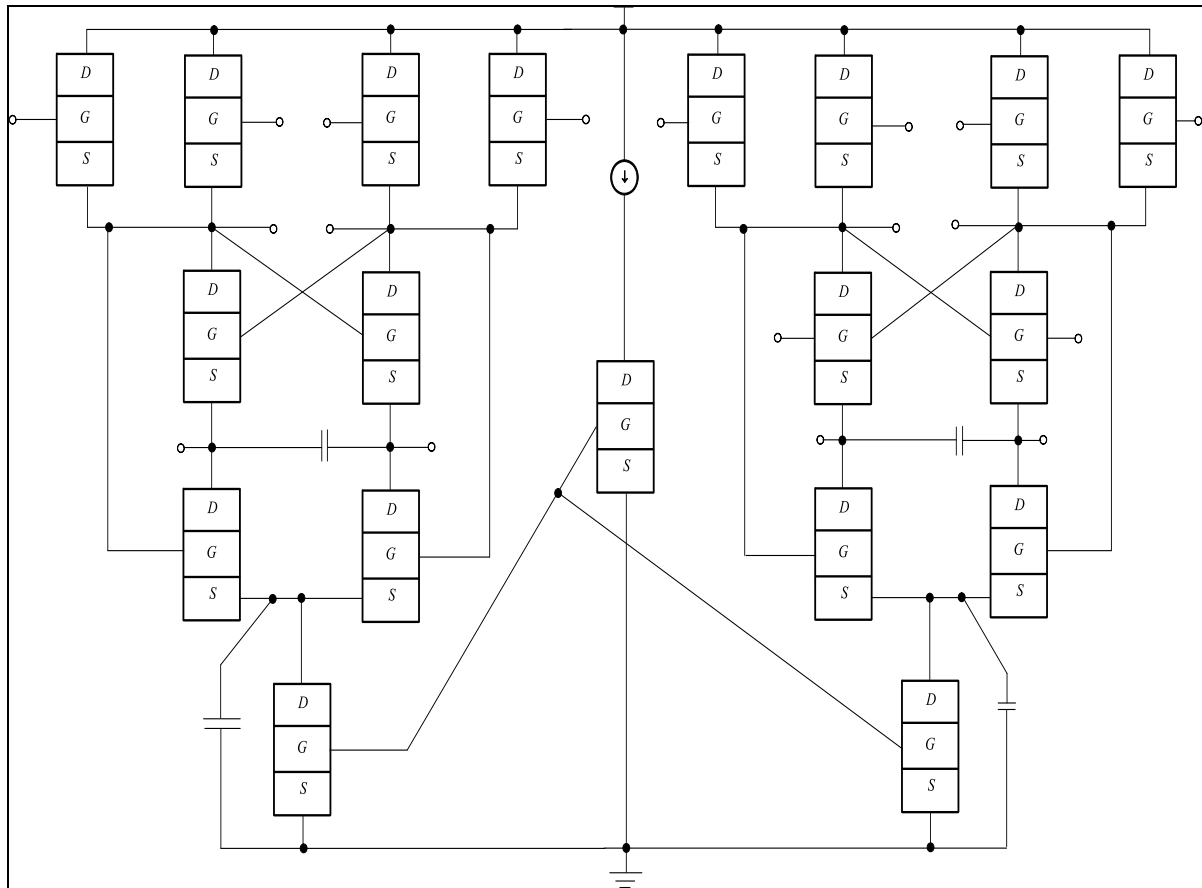
Fig 1a: Structure of the considered oscillator [19]
