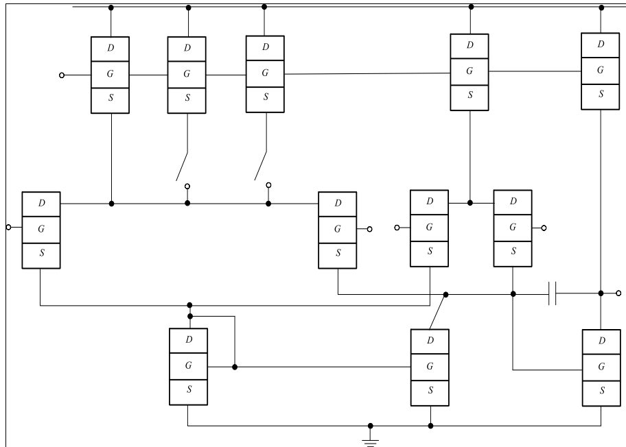
Fig 1a: Structure of the considered instrumentation amplifier [19]
