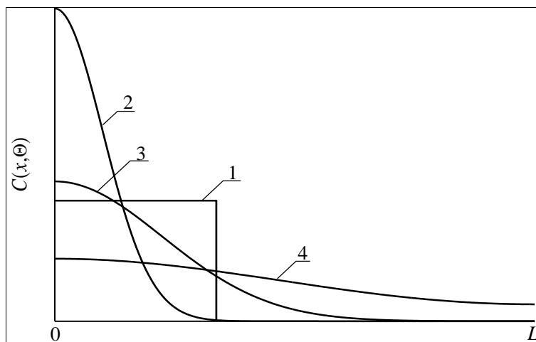
Fig 4: Spatial distributions of dopant in heterostructure after dopant infusion. Curve 1 is idealized distribution of dopant. Curves 2-4 are real distributions of dopant for different values of annealing time. Increasing of number of curve corresponds to increasing of annealing time
