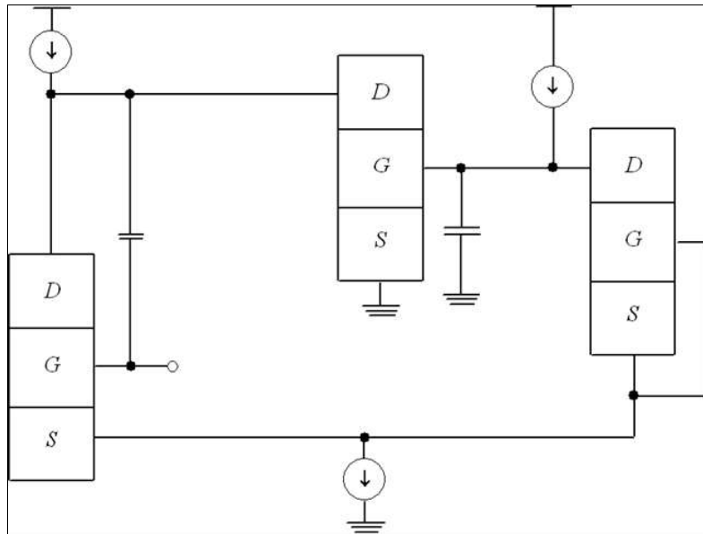
Fig 1a: Structure of the considered filter [15]
